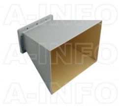
LB-650-10-A Standard Gain Horn Antenna 1.12-1.7GHz 10dB Gain Rectangular Waveguide Interface
